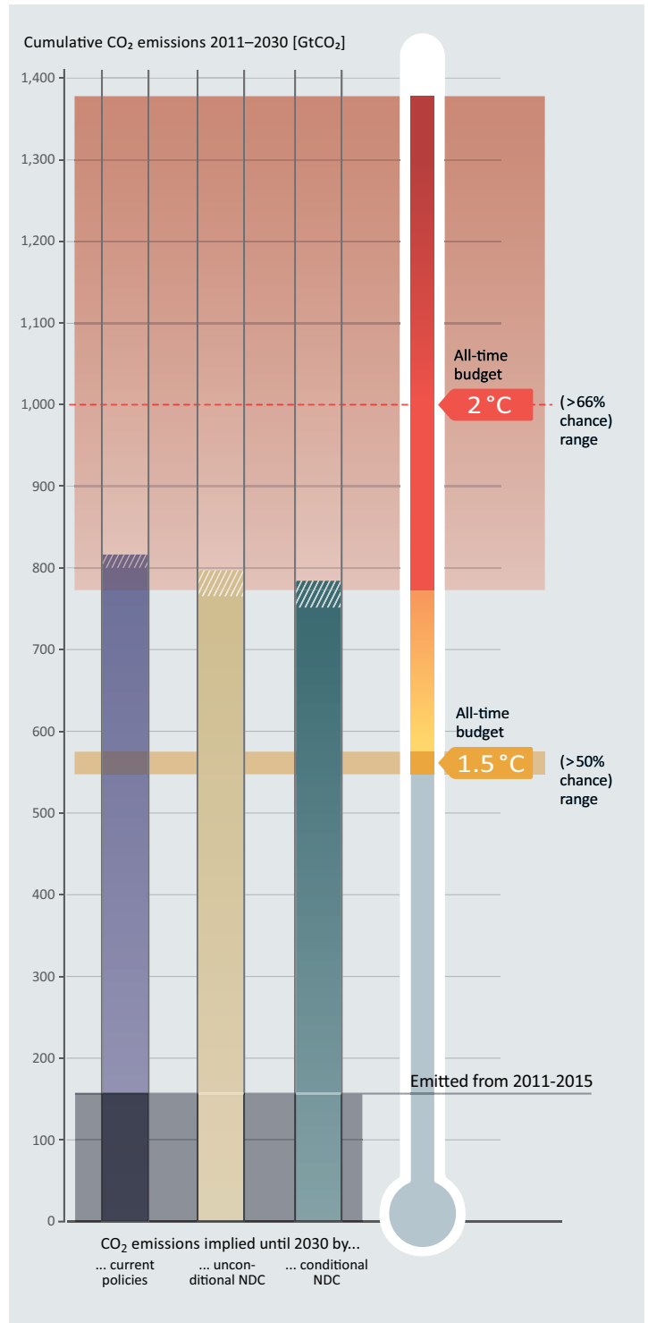
Figure 3.2: Comparison of projected emissions by 2030 and all-time 1.5°C and 2°C carbon budgets.
