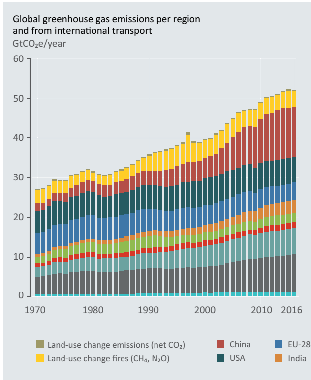
Figure ES.1.a: Global greenhouse gas emissions for top six emitting countries and regions (excluding land use, land-use change and forestry), international transport emissions, and land use, land-use change and forestry emissions.
