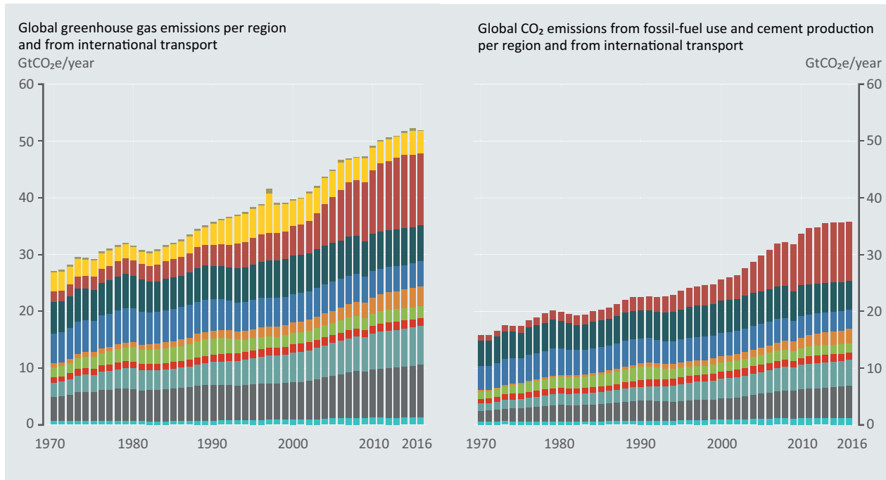
Figure 2.1.a: Global greenhouse gas emissions for top six emitting countries and regions (excluding land use, land-use change and forestry), international transport emissions, and land use, land-use change and forestry emissions.
