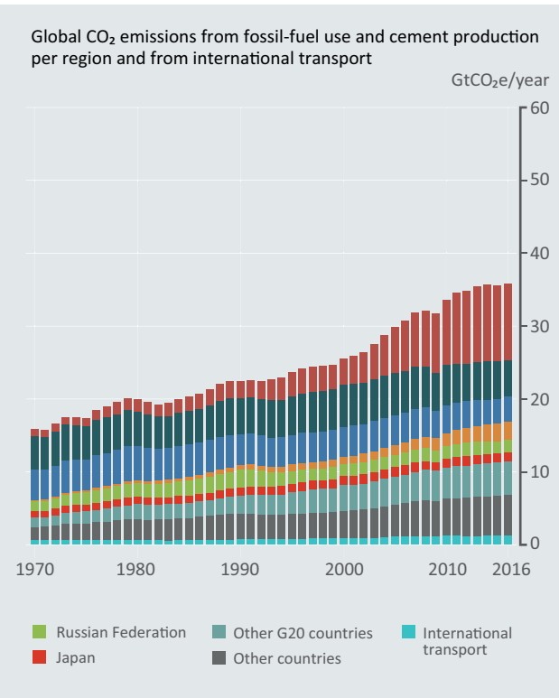
Figure ES.1.b: Global carbon dioxide emissions per region from fossil fuel use, cement production and other processes.
